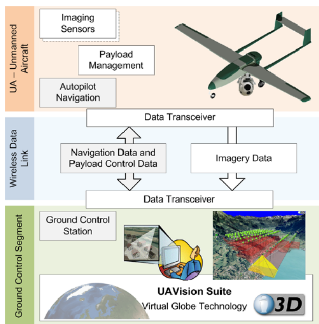
Figure 2: UAVision system architecture and hardware components
