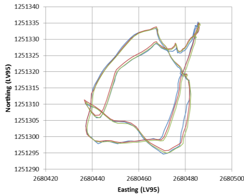
Figure 5. Footprints of the Falcon trajectories from LGO GPS post-processing, GrafNav GPS post-processing and tracking data (total station).
